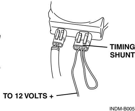
Figure 6.9 – Timing Shunt
